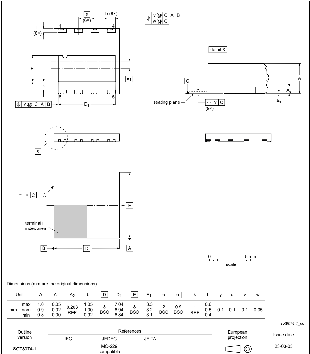
Fig. 1. Package outline DFN8080-8 (SOT8074-1)
