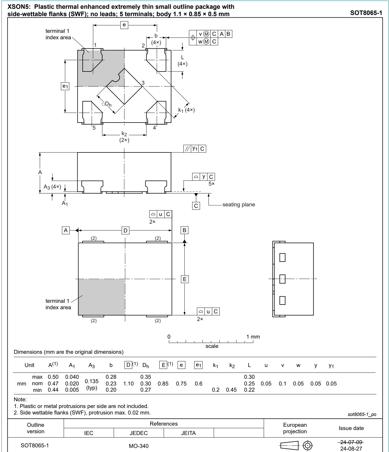
Fig. 1. Package outline XSON5 (SOT8065-1)
