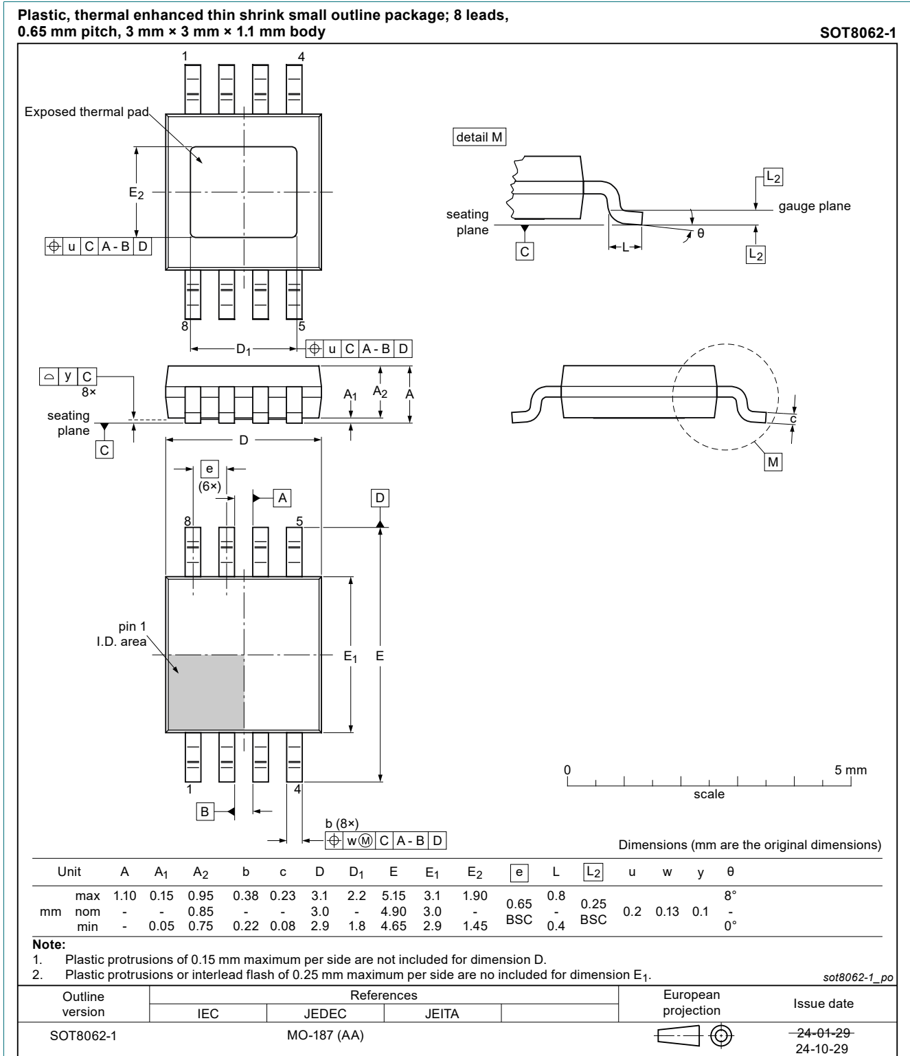
Fig. 1. Package outline HTSSOP (SOT8062-1)
