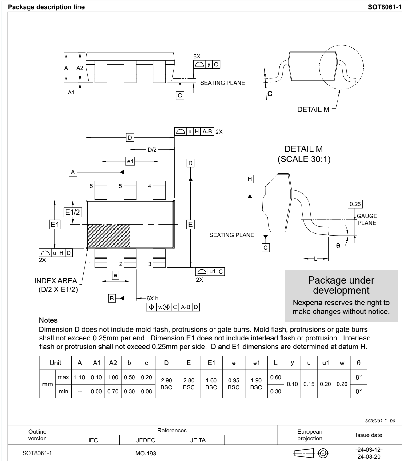
Fig. 1. Package outline TSSOP6 (SOT8061-1)
