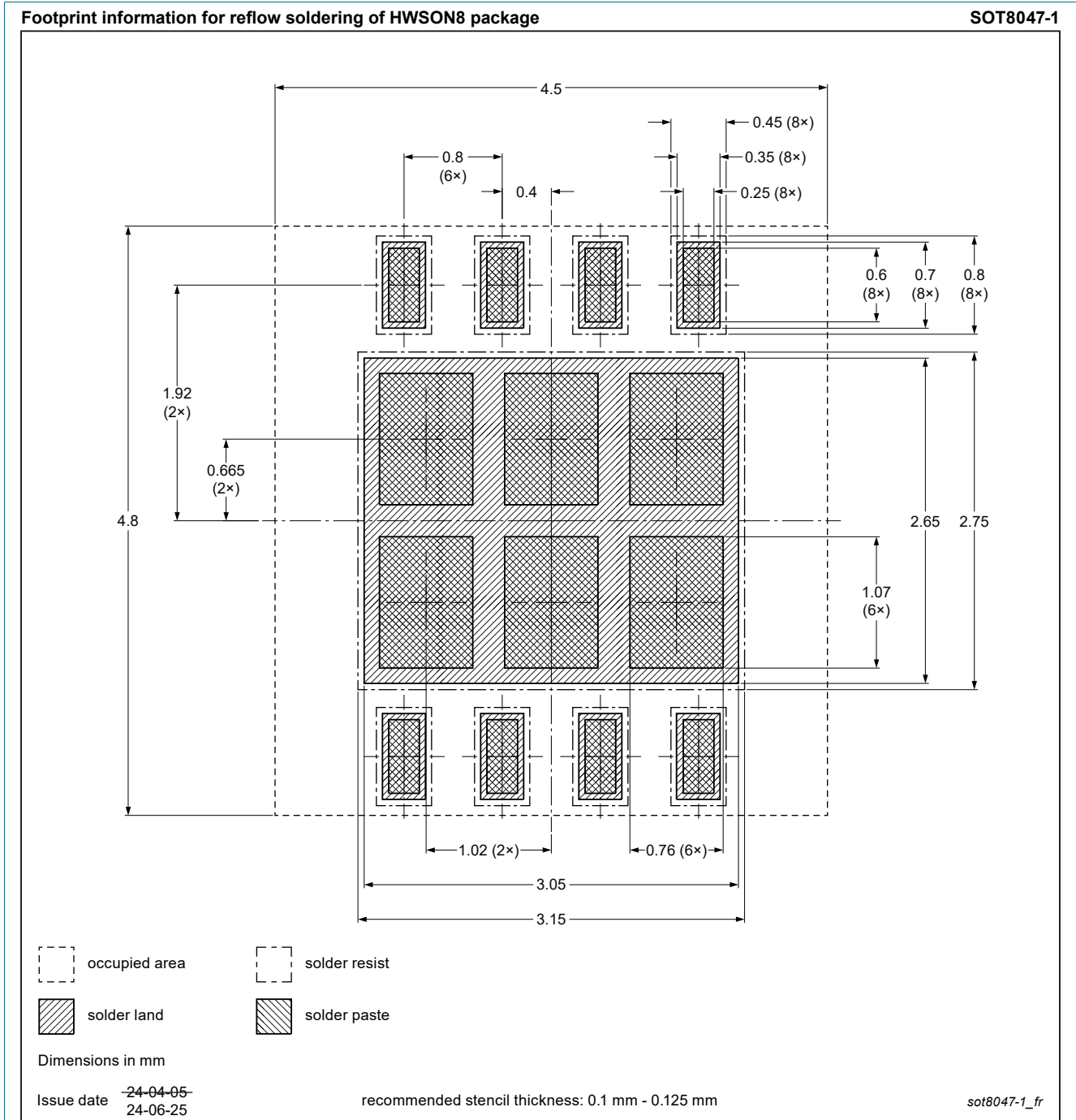
Fig. 2. Reflow soldering footprint for HWSO8 (SOT8047-1)
