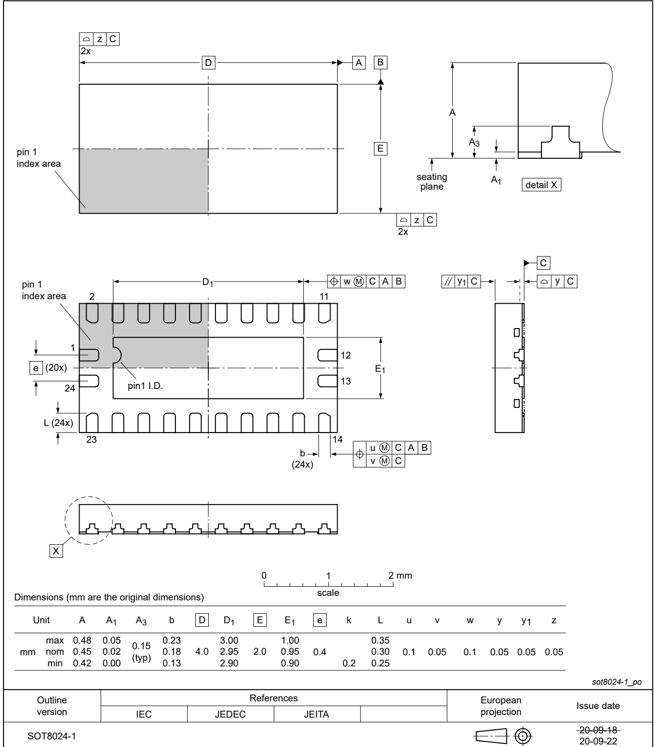
Fig. 1. Package outline DHXQFN (SOT8024-1)
