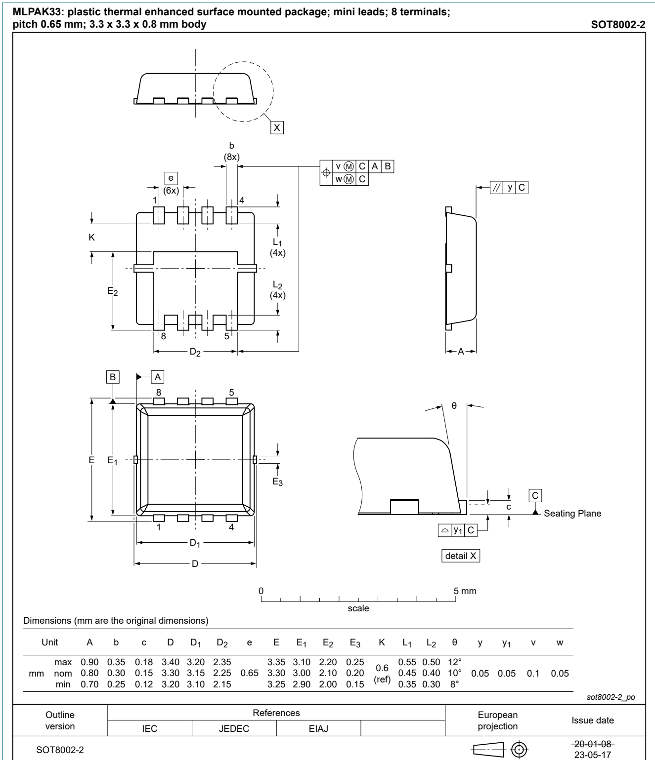
Fig. 1. Package outline MLPAK33 (SOT8002-2)
