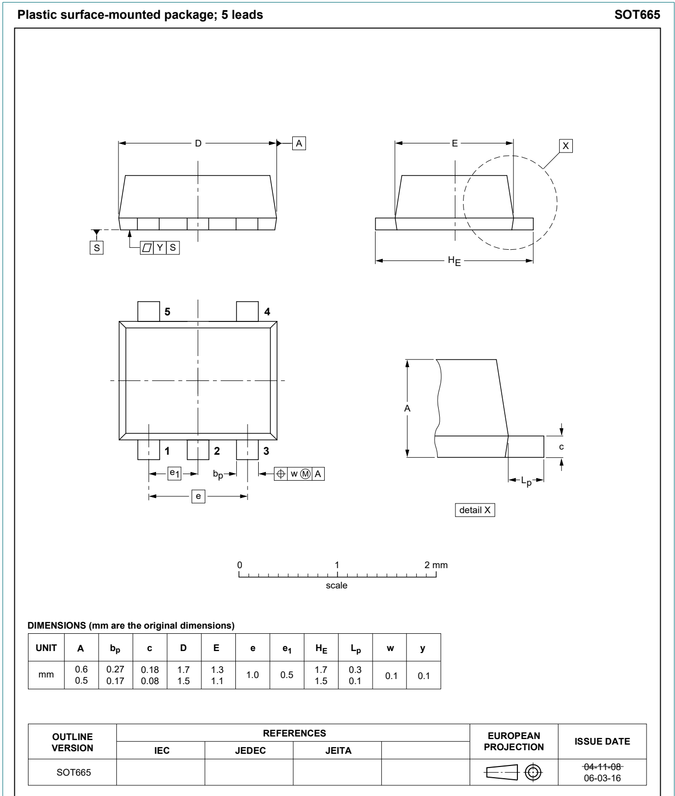
Fig. 1. Package outline SOT665
