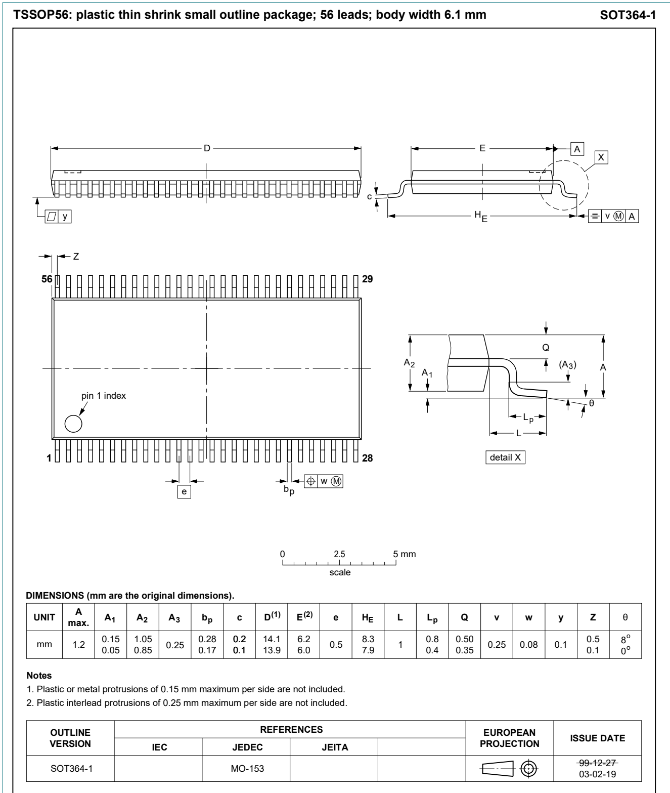
Fig. 1. Package outline TSSOP56 (SOT364-1)
