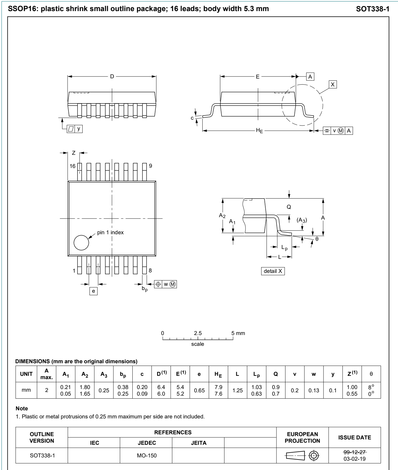
Fig. 1. Package outline SSOP16 (SOT338-1)
