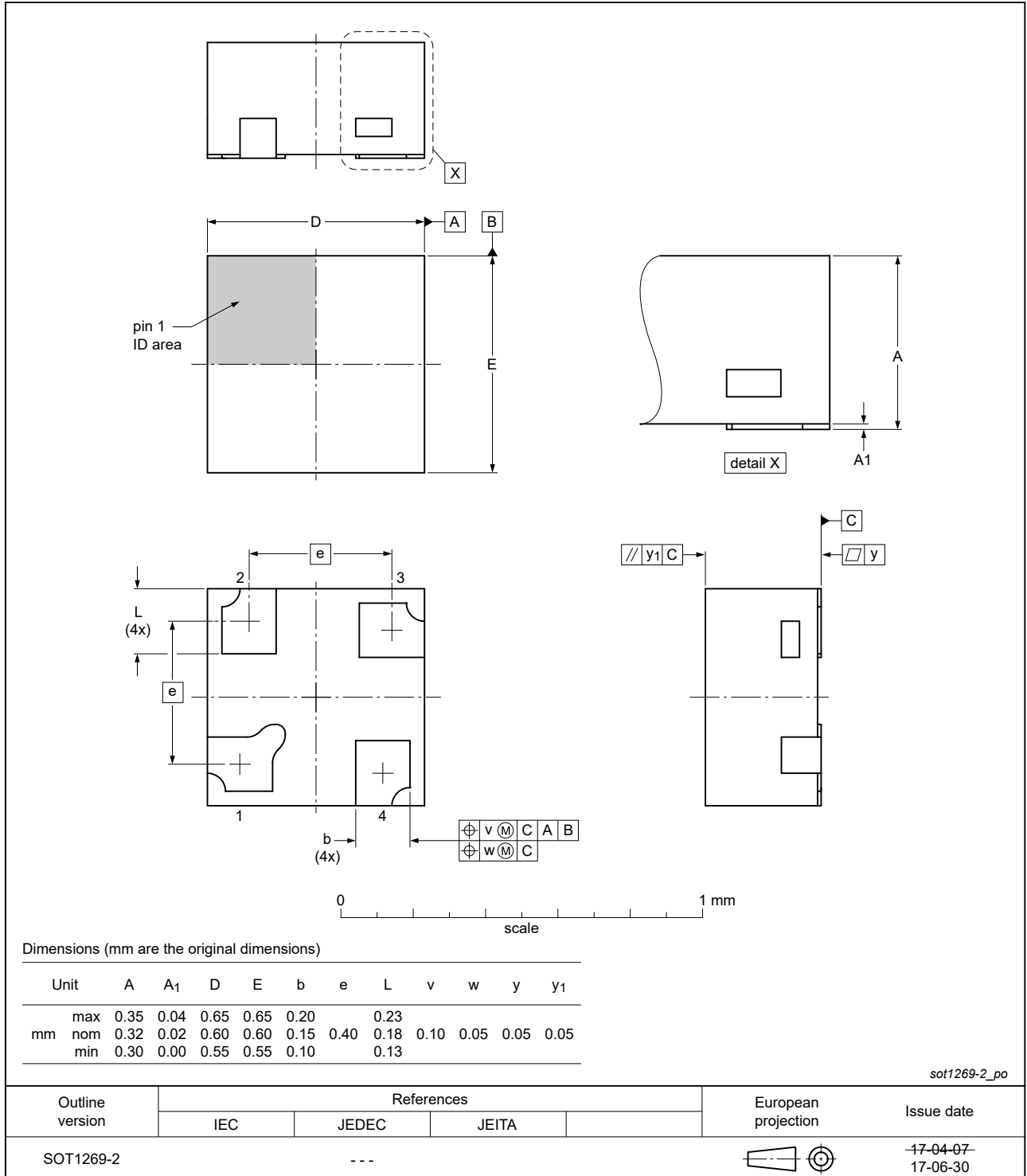
Fig. 1. Package outline X2SON4 (SOT1269-2)
