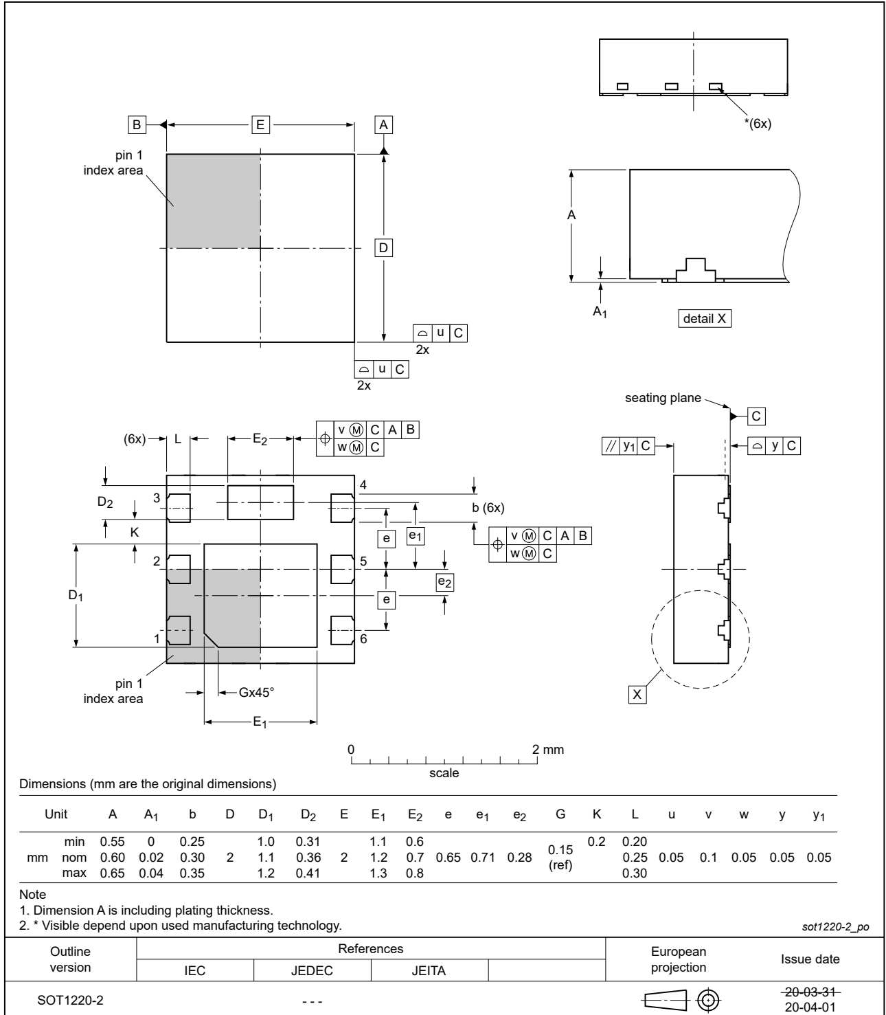
Fig. 1. Package outline DFN2020M-6 (SOT1220-2)
