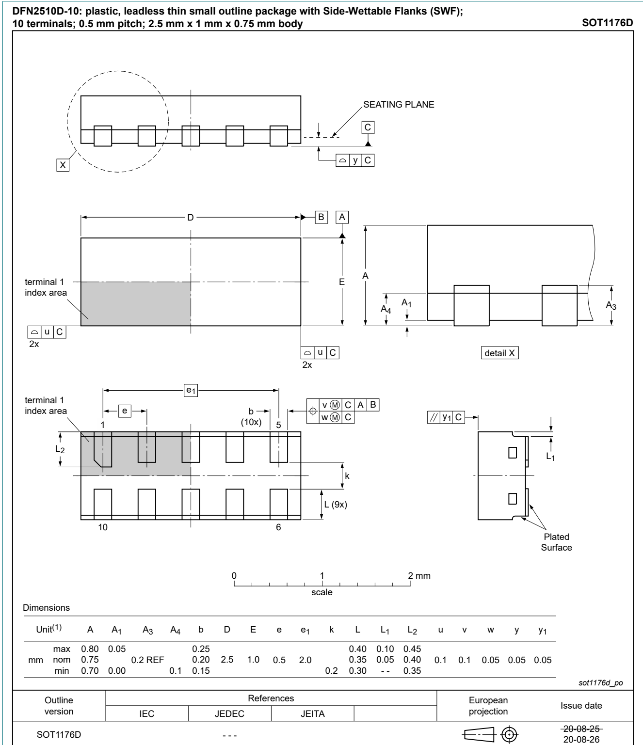
Fig. 1. Package outline DFN2510D (SOT1176D)
