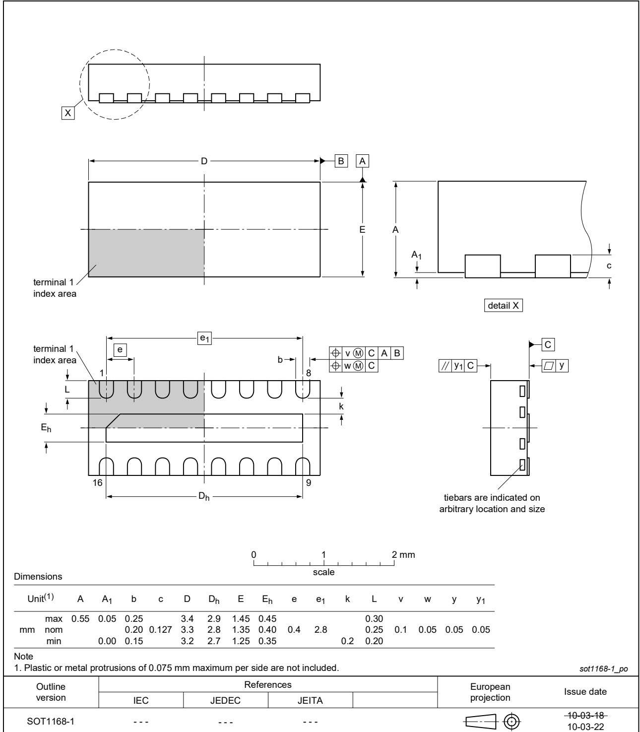
Fig. 1. Package outline DFN3314-16 (SOT1168-1)
