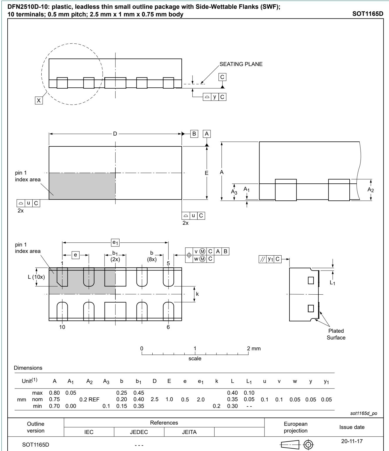
Fig. 1. Package outline DFN2510D (SOT1165D)
