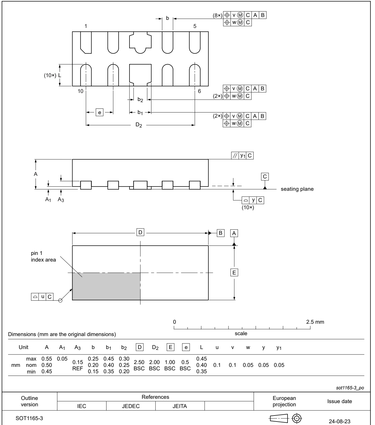
Fig. 1. Package outline DFN2510-10 (SOT1165-3)
