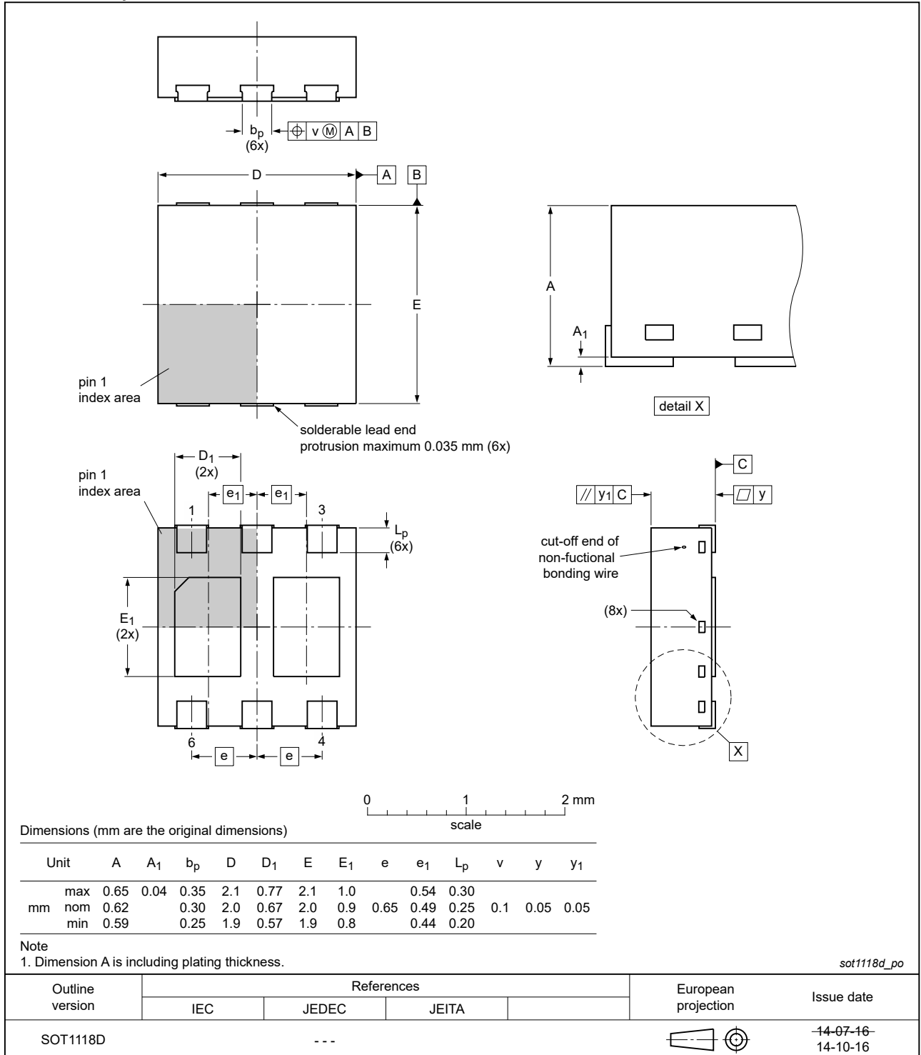
Fig. 1. Package outline DFN2020D-6 (SOT1118D)
