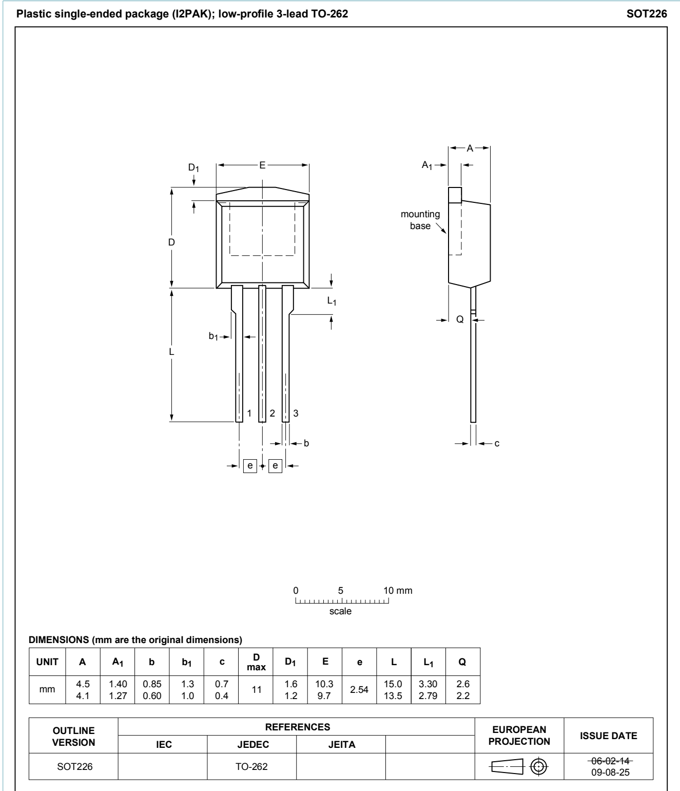
Fig. 1. Package outline I2PAK (SOT226)
