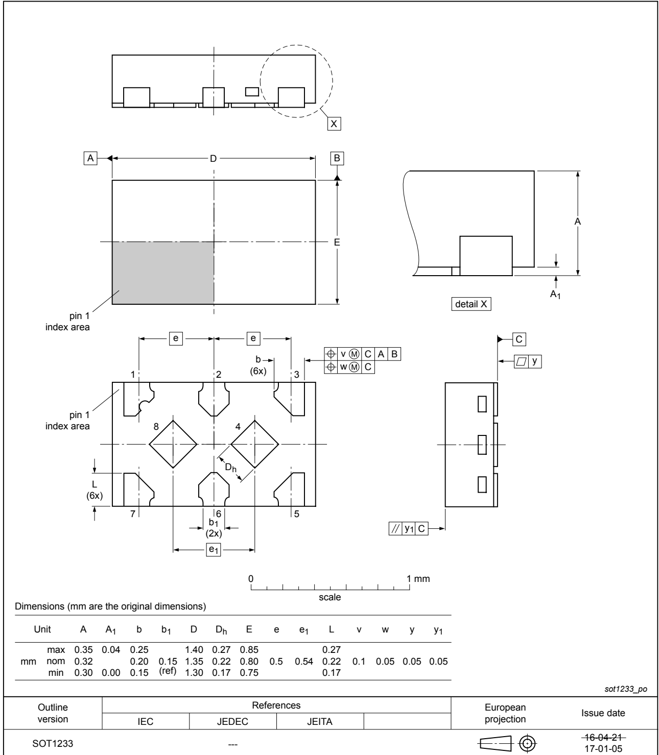
Fig. 1. Package outline X2SON8 (SOT1233)
