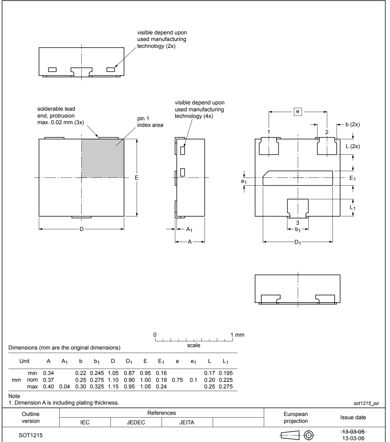
Fig. 1. Package outline DFN1010D-3 (SOT1215)
