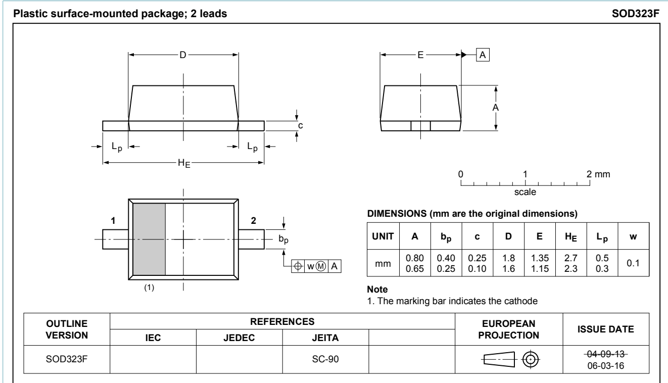
Fig. 1. Package outline SC-90 (SOD323F)
