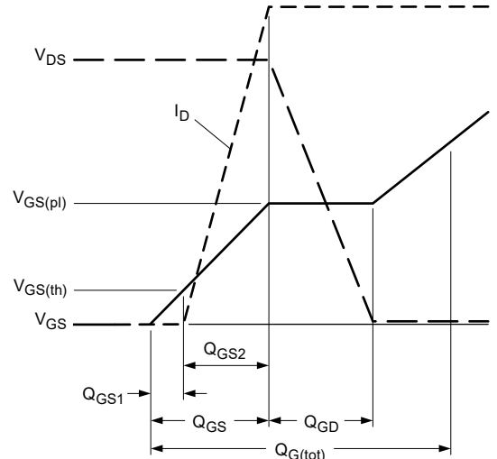
Fig. 15. Gate charge waveform definitions
