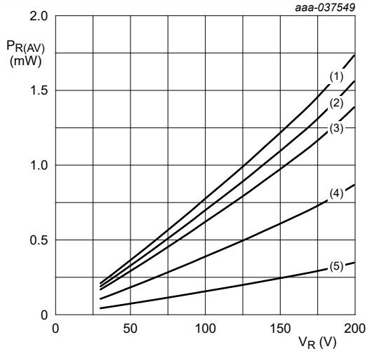
T_j = 175\text{ }^\circ\text{C} (1) \delta = 1 (2) \delta = 0.9 (3) \delta = 0.8 (4) \delta = 0.5 (5) \delta = 0.2
