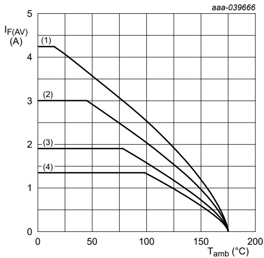
FR4 PCB, mounting pad for cathode 1\text{ cm}^2 T_j = 175\text{ }^\circ\text{C} (1) \delta = 1 (2) \delta = 0.5 ; f = 20\text{ kHz} (3) \delta = 0.2 ; f = 20\text{ kHz} (4) \delta = 0.1 ; f = 20\text{ kHz}
