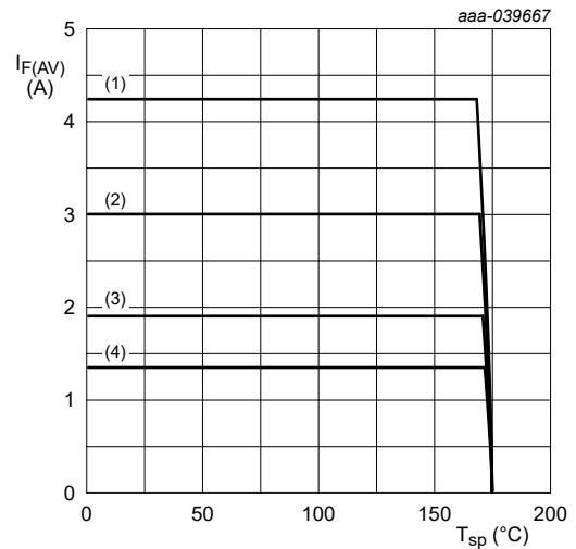
T_j = 175\text{ }^\circ\text{C} (1) \delta = 1 (2) \delta = 0.5 ; f = 20\text{ kHz} (3) \delta = 0.2 ; f = 20\text{ kHz} (4) \delta = 0.1 ; f = 20\text{ kHz}
