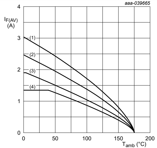
FR4 PCB, standard footprint T_j = 175\text{ }^\circ\text{C} (1) \delta = 1 (2) \delta = 0.5 ; f = 20\text{ kHz} (3) \delta = 0.2 ; f = 20\text{ kHz} (4) \delta = 0.1 ; f = 20\text{ kHz}
