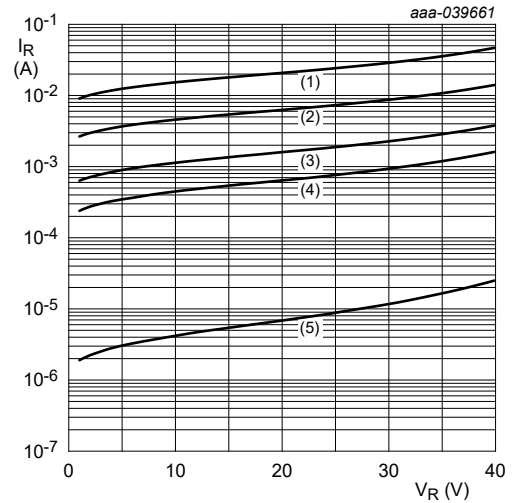
pulsed condition (1) T_j = 150\text{ }^\circ\text{C} (2) T_j = 125\text{ }^\circ\text{C} (3) T_j = 100\text{ }^\circ\text{C} (4) T_j = 85\text{ }^\circ\text{C} (5) T_j = 25\text{ }^\circ\text{C}
