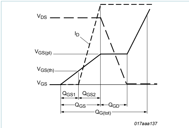
Fig. 28. MOSFET transistor: Gate charge waveform definitions
