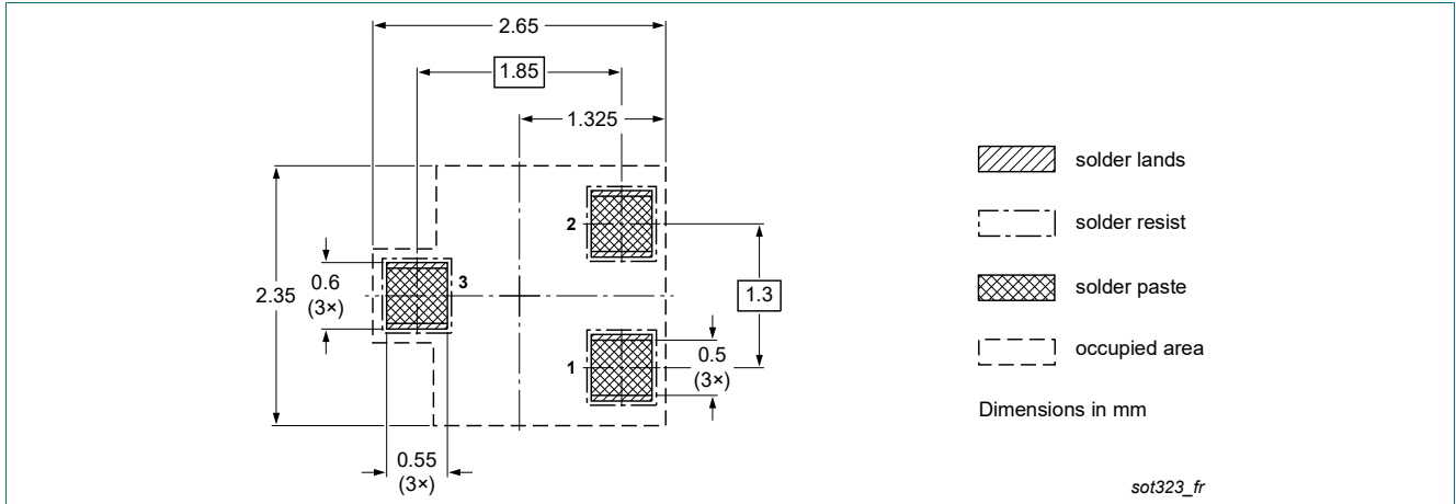
Fig. 9. Reflow soldering footprint for SC-70 (SOT323)
