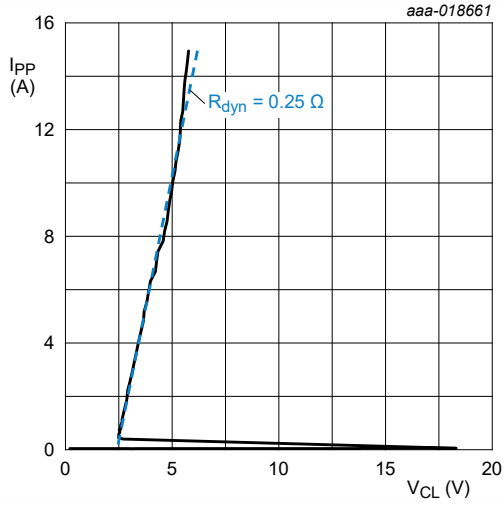
Fig. 9. Dynamic resistance with positive clamping voltage; typical values
