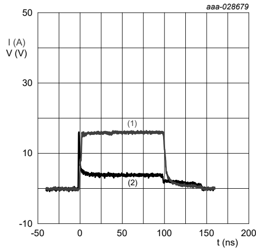
Fig. 9. Dynamic resistance with positive clamping; typical values
