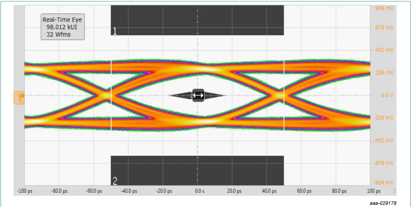
Fig. 6. USB 3.2 eye diagram, test board with device; typical values
