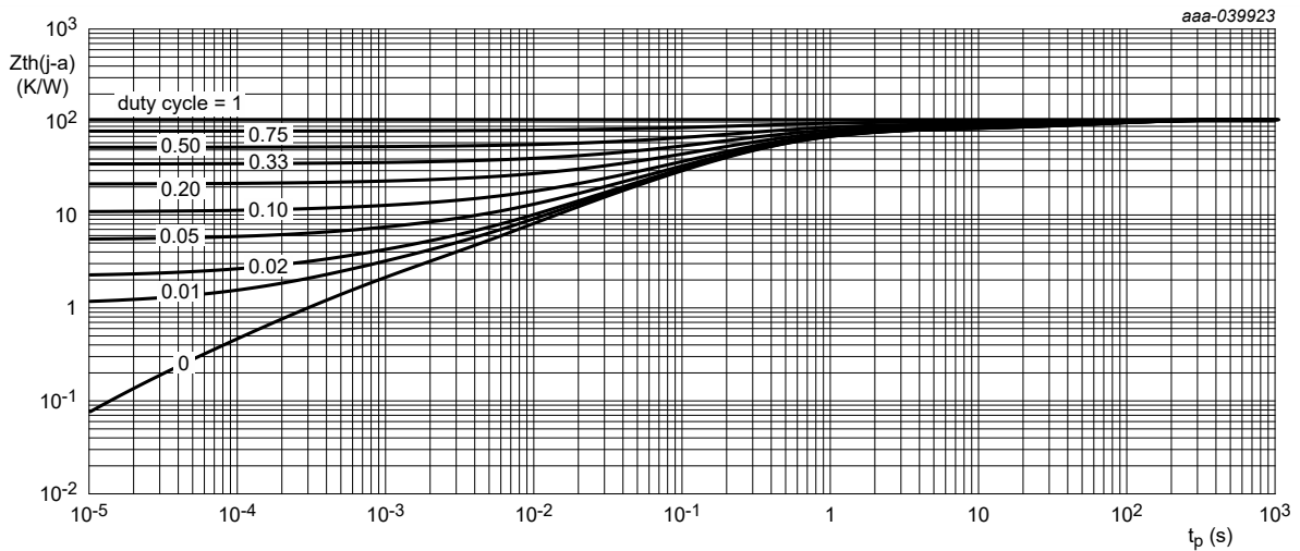
FR4 PCB, 4-layer, tin-plated, mounting pad for collector 1 cm 2
