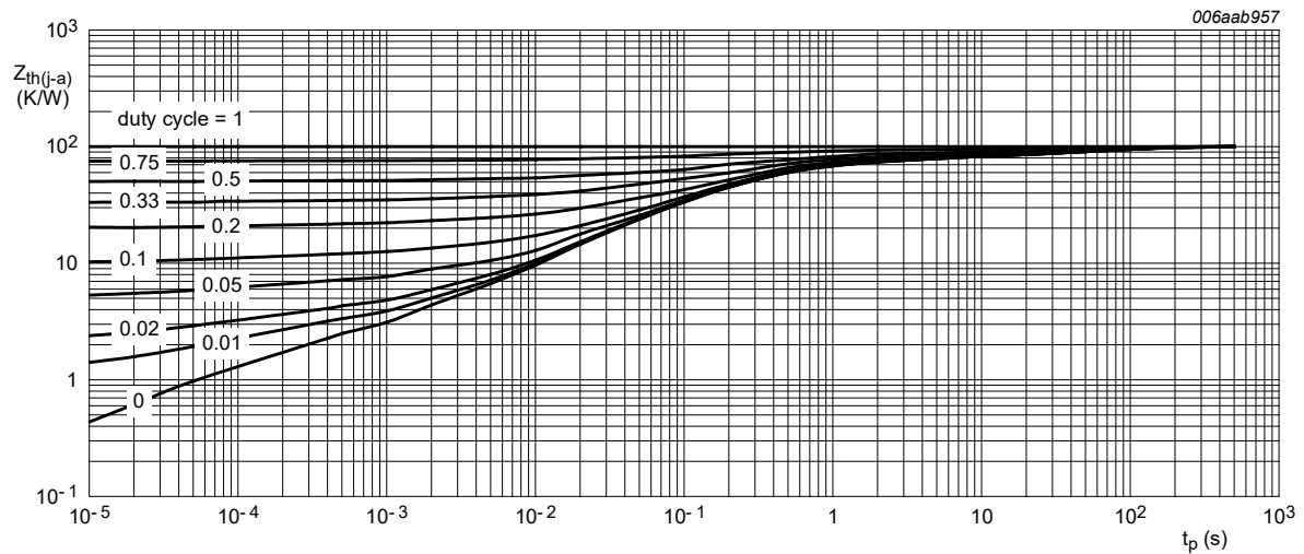
Ceramic PCB, Al 2 O 3 , single-sided, 35 μm copper, tin-plated and standard footprint
