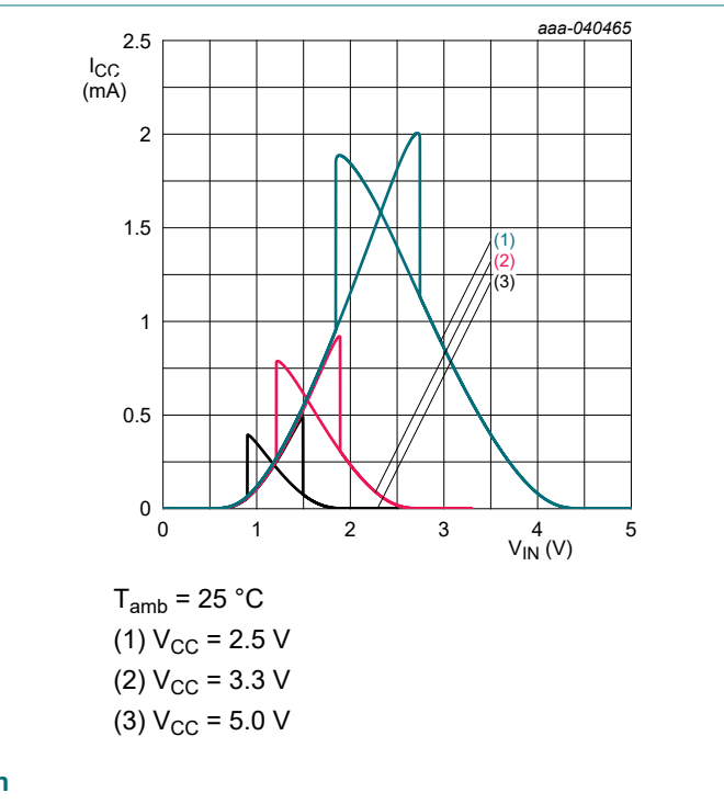
Fig. 5. Typical transfer characteristics for data inputs A_n
