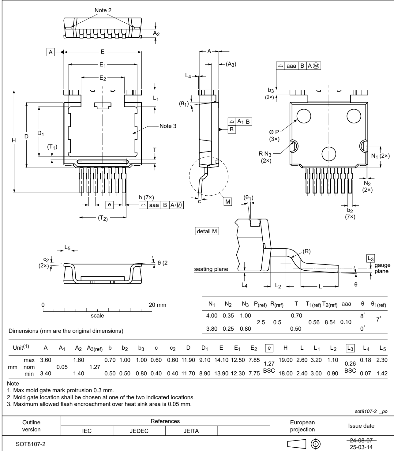
Fig. 28. Package outline X.PAK (SOT8107-2)
