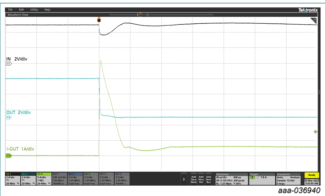
Fig. 8. Hard short
