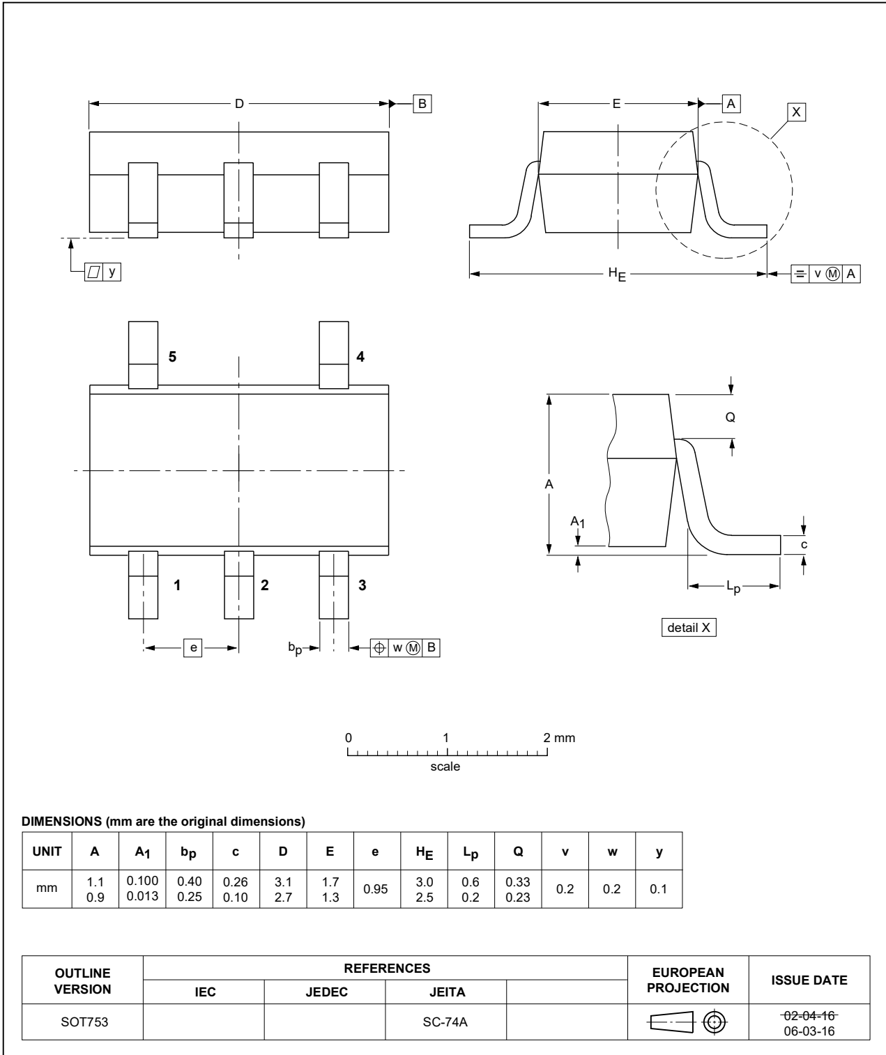
Fig. 21. Package outline SOT753 (SC-74A)
