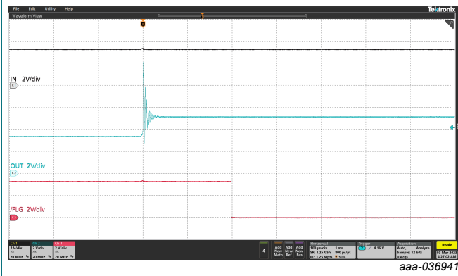
Fig. 9. Reverse voltage blocking
