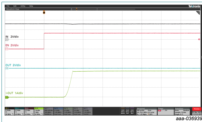
Fig. 7. Enable to short
