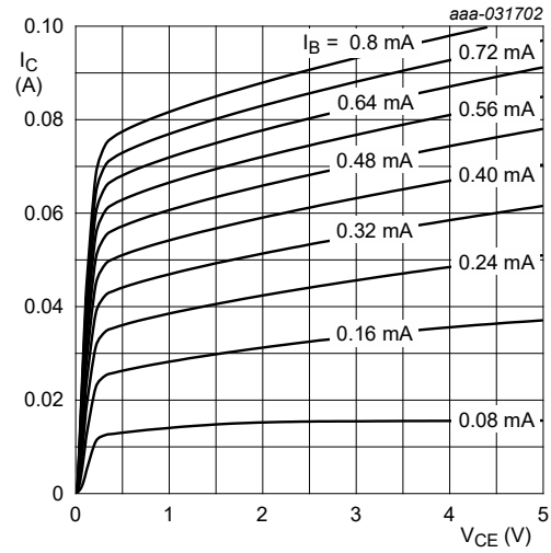
Fig. 16. NHUMD2-Q, TR1 (NPN): Collector current as a function of collector-emitter voltage; typical values
