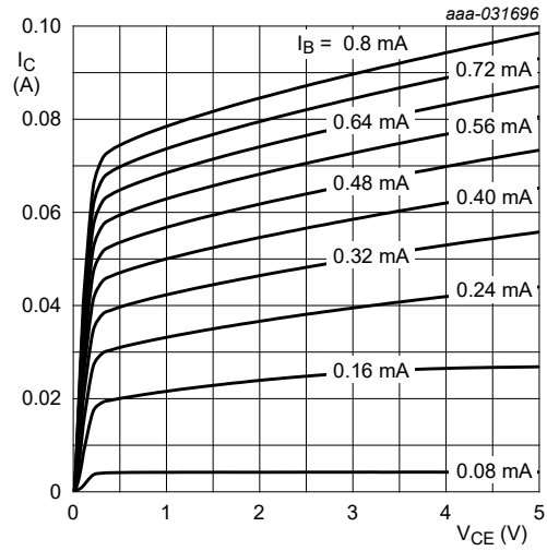
Fig. 4. NHUMD3-Q, TR1 (NPN): Collector current as a function of collector-emitter voltage; typical values
