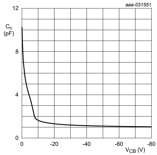
Fig. 38. NHUMD12-Q, TR2 (PNP): Collector capacitance as a function of collector-base voltage; typical values of built-in transistor
