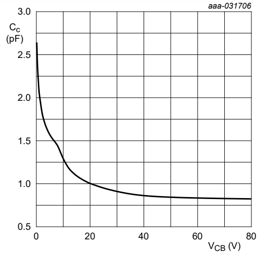
Fig. 20. NHUMD2-Q, TR1 (NPN): Collector capacitance as a function of collector-base voltage; typical values
