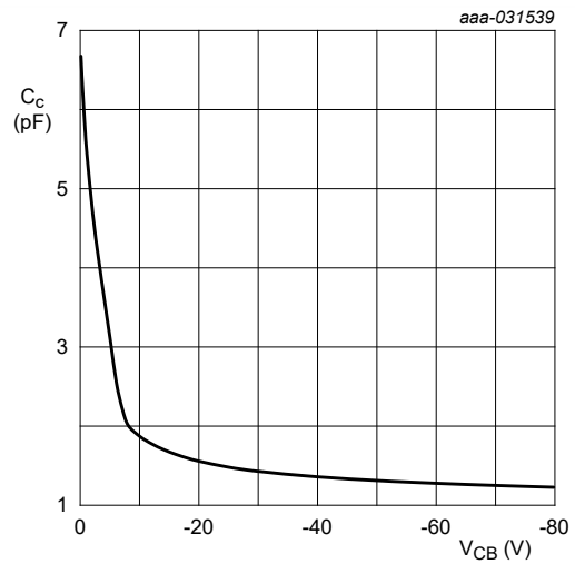
Fig. 14. NHUMD3-Q, TR2 (PNP): Collector capacitance as a function of collector-base voltage; typical values
