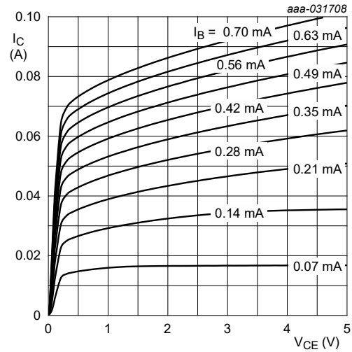
Fig. 28. NHUMD12-Q, TR1 (NPN): Collector current as a function of collector-emitter voltage; typical values
