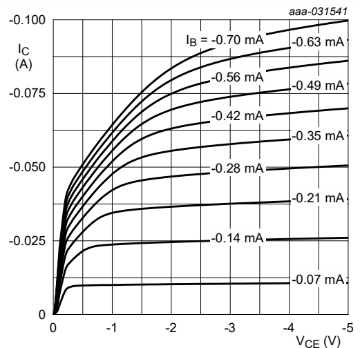
Fig. 22. NHUMD2-Q, TR2 (PNP): Collector current as a function of collector-emitter voltage; typical values
