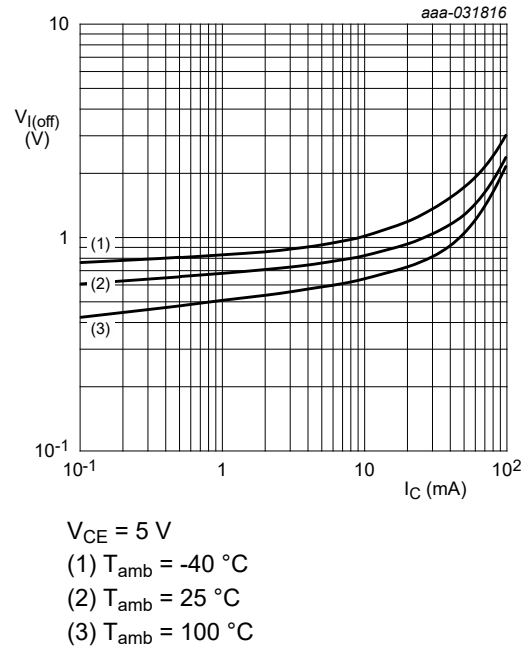
Fig. 7. NHDTC123JU-Q: Off-state input voltage as a function of collector current; typical values
