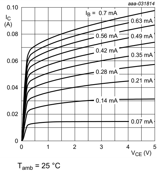
Fig. 5. NHDTC123JU-Q: Collector current as a function of collector-emitter voltage; typical values
