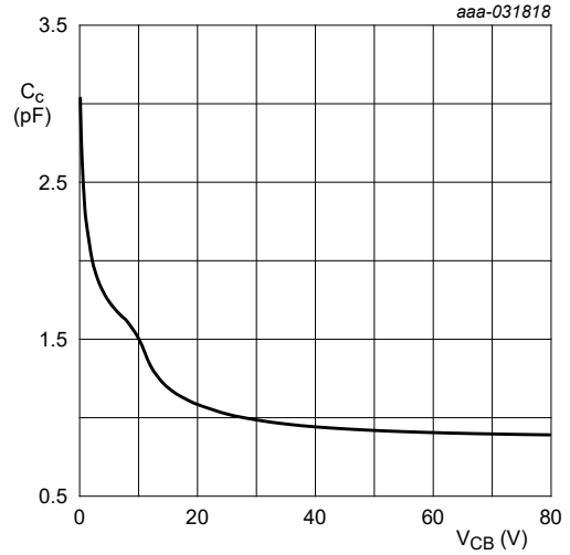
Fig. 9. NHDTC123JT-Q: Collector capacitance as a function of collector-base voltage; typical values
