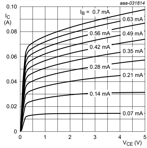
Fig. 5. NHDTC123JT-Q: Collector current as a function of collector-emitter voltage; typical values
