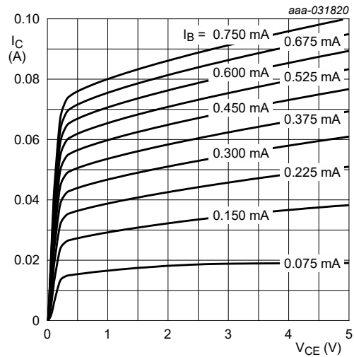
Fig. 11. NHDTC143ZT-Q: Collector current as a function of collector-emitter voltage; typical values
