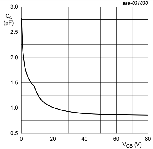
Fig. 21. NHDTC114YT-Q: Collector capacitance as a function of collector-base voltage; typical values
