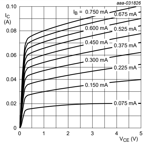
Fig. 17. NHDTC114YT-Q: Collector current as a function of collector-emitter voltage; typical values
