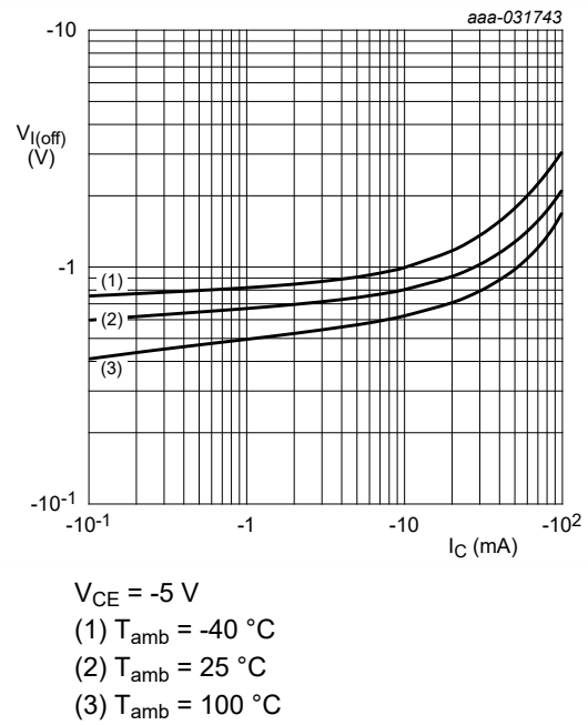
Fig. 7. NHDTA123JU-Q: Off-state input voltage as a function of collector current; typical values
