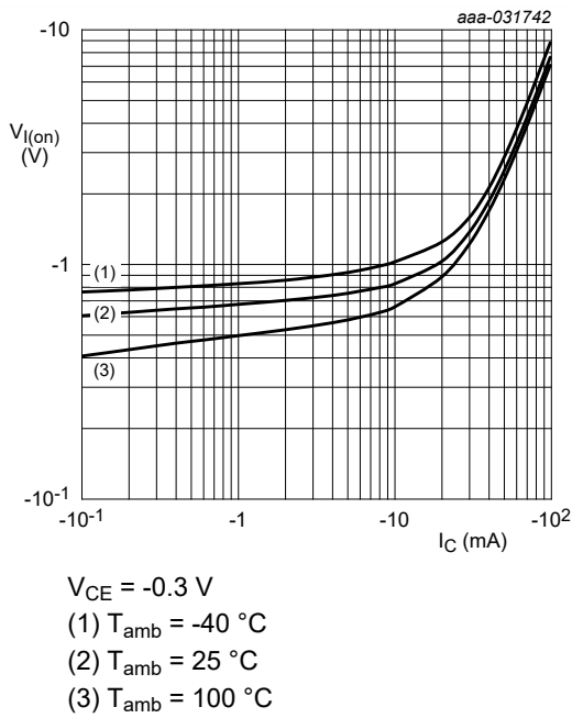
Fig. 6. NHDTA123JU-Q: On-state input voltage as a function of collector current; typical values
