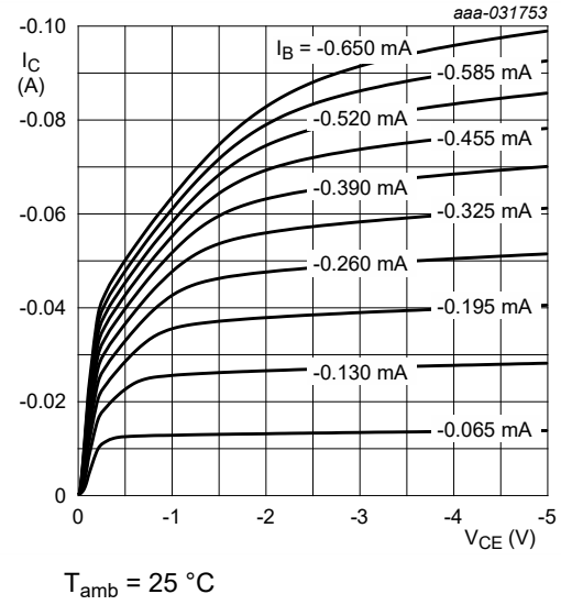
Fig. 17. NHDTA114YU-Q: Collector current as a function of collector-emitter voltage; typical values
