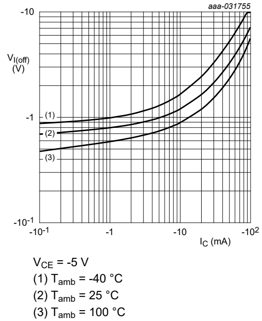
Fig. 19. NHDTA114YU-Q: Off-state input voltage as a function of collector current; typical values
