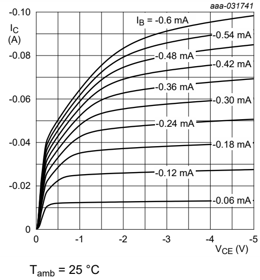
Fig. 5. NHDTA123JU-Q: Collector current as a function of collector-emitter voltage; typical values
