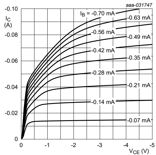
Fig. 11. NHDTA143ZU-Q: Collector current as a function of collector-emitter voltage; typical values
