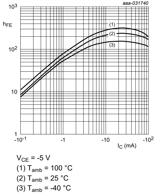
Fig. 4. NHDTA123JU-Q: DC current gain as a function of collector current; typical values
