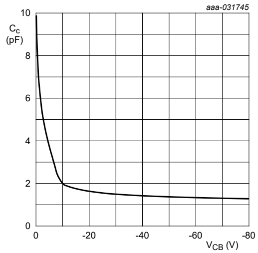
Fig. 9. NHDTA123JU-Q: Collector capacitance as a function of collector-base voltage; typical values
