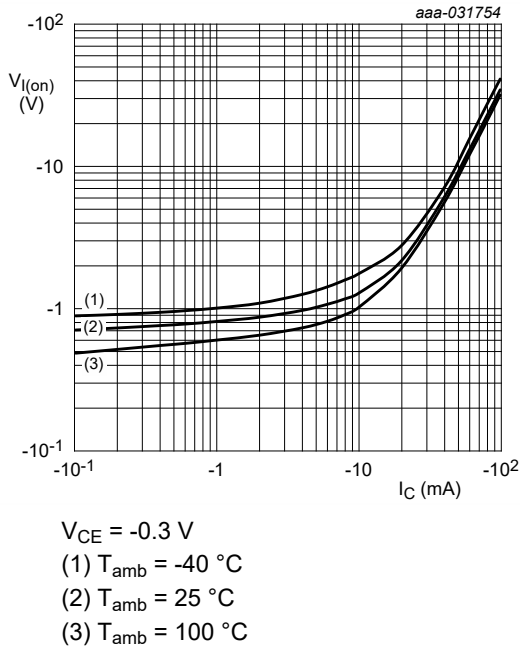
Fig. 18. NHDTA114YU-Q: On-state input voltage as a function of collector current; typical values
