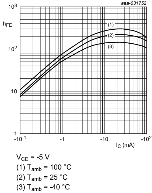
Fig. 16. NHDTA114YU-Q: DC current gain as a function of collector current; typical values
