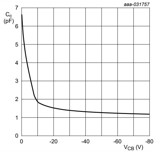
Fig. 21. NHDTA114YU-Q: Collector capacitance as a function of collector-base voltage; typical values
