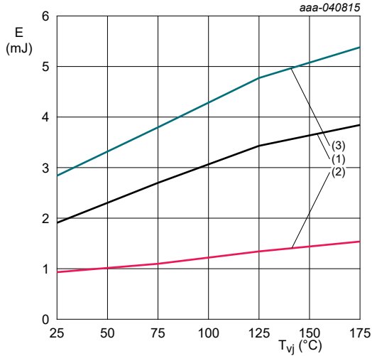
V_{GE} = 15 \text{ V to } 0 \text{ V}; V_{CC} = 400 \text{ V}; I_C = 60 \text{ A}; R_{G(on)} = 10 \text{ } \Omega; R_{G(off)} = 10 \text{ } \Omega (1) E_{on} (2) E_{off} (3) E_{ts}
