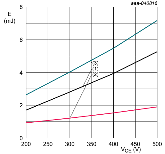
V_{GE} = 15 \text{ V to } 0 \text{ V}; I_C = 60 \text{ A}; R_{G(on)} = 10 \text{ } \Omega; R_{G(off)} = 10 \text{ } \Omega; T_{vj} = 175 \text{ } ^\circ\text{C} (1) E_{on} (2) E_{off} (3) E_{ts}
