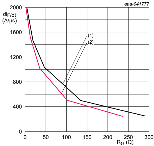
V_R = 400 \text{ V}; I_F = 60 \text{ A} (1) T_{vj} = 25 \text{ } ^\circ\text{C} (2) T_{vj} = 175 \text{ } ^\circ\text{C}
