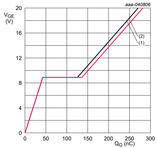
I_C = 60 A (1) V_{CE} = 130 V (2) V_{CE} = 520 V
