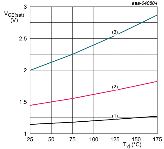
V_{GE} = 15 V (1) I_C = 30 A (2) I_C = 60 A (3) I_C = 120 A
