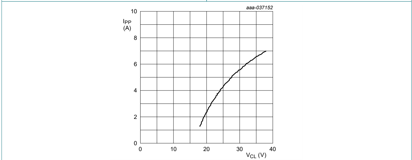
Fig. 5. Positive clamping voltage (8/20 \mu\text{s} pulse); typical values
