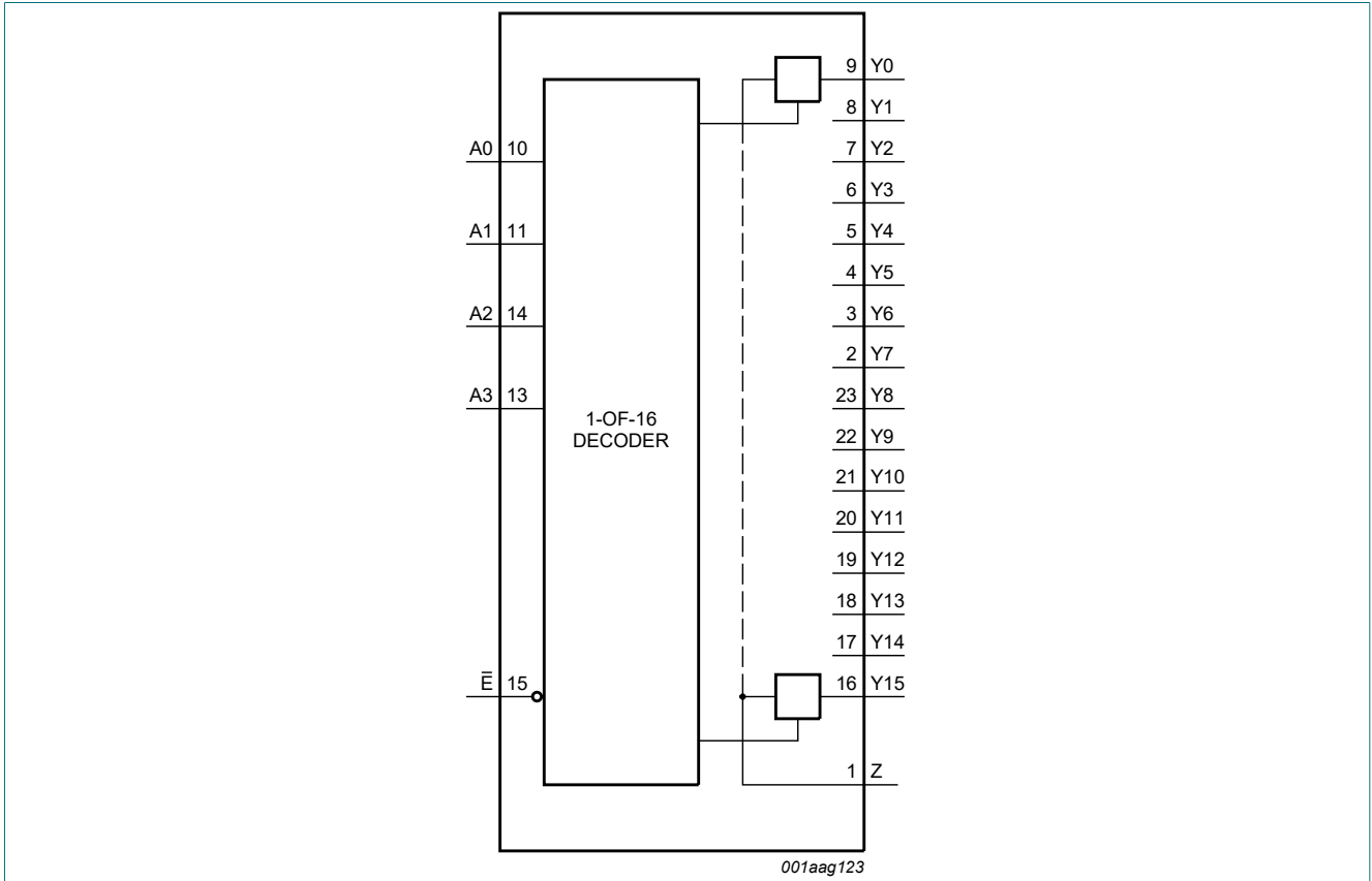
Fig. 1. Functional diagram
