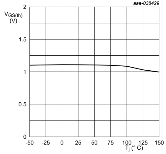
Fig. 7. Gate-source threshold voltage as a function of junction temperature; typical values
