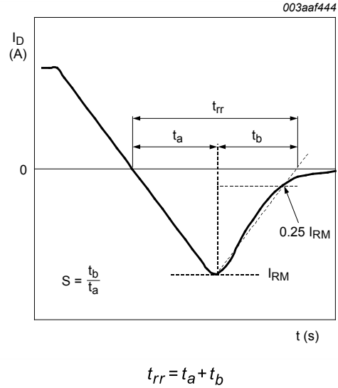
Fig. 17. Reverse recovery waveform definitions
