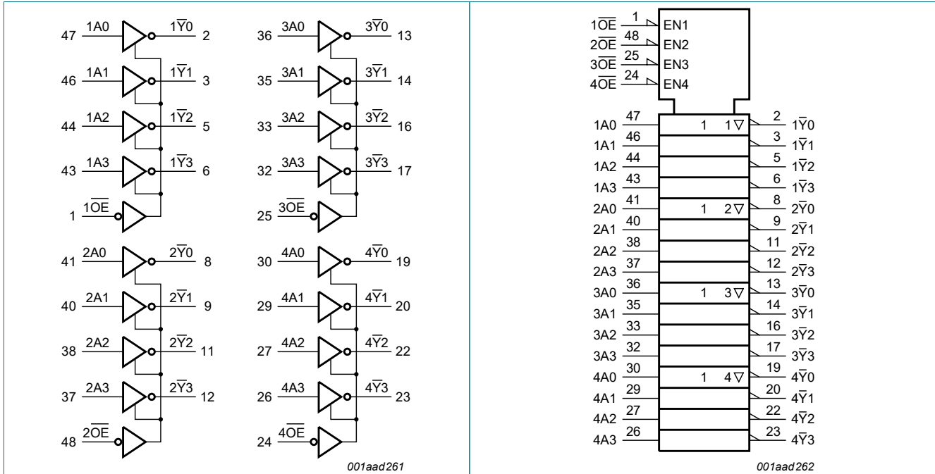
Fig. 1. Logic symbol
