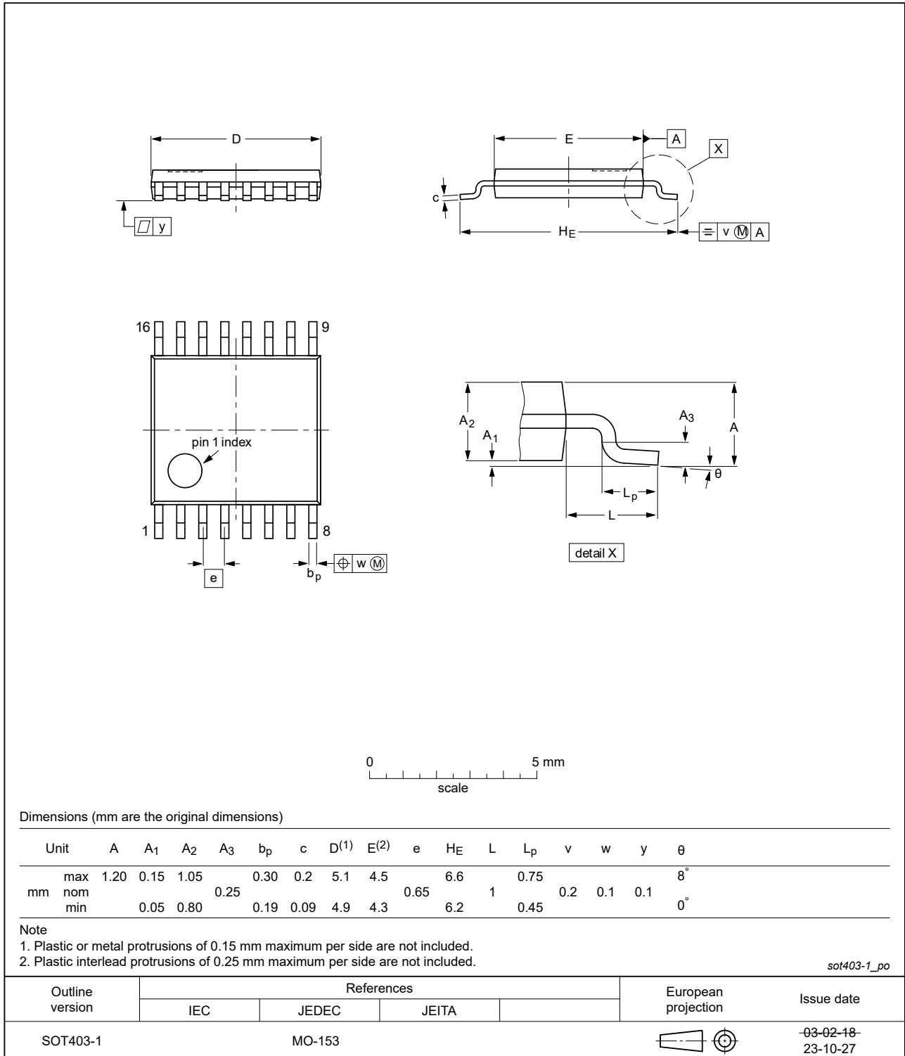
Fig. 35. Package outline SOT403-1 (TSSOP16)
