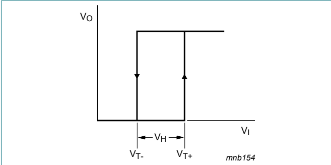
Fig. 4. Transfer characteristics
