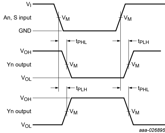
Measurement points are given in Table 9 . V_{OL} and V_{OH} are typical voltage output levels that occur with the output load.
