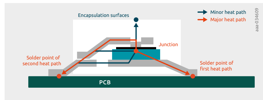
Figure 52 | Cross section of a typical clip bonded flat power package – heat paths highlighted.
