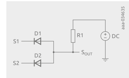
Figure 116 | Diodes AND function.
